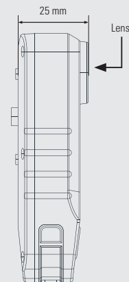
View on Right Face
